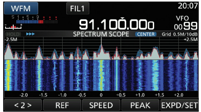
Figure 3 — Spectrum of FM broadcast signals.
